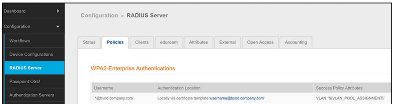
FIGURE 57 Confirming VLAN Variable in RADIUS Server Policies
