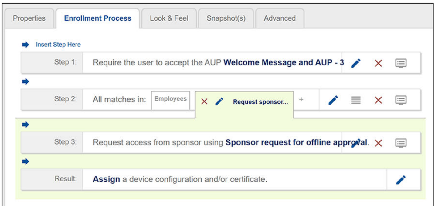
FIGURE 76 Sample Workflow That Uses the "Request Access for a User Offline" Plug-in
