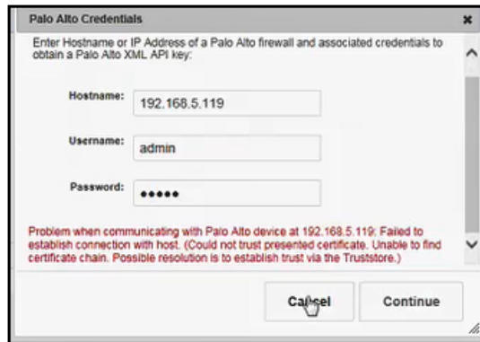
FIGURE 113 Possible Error Message While Cloudpath Tries to Connect to Palo Alto Firewall
