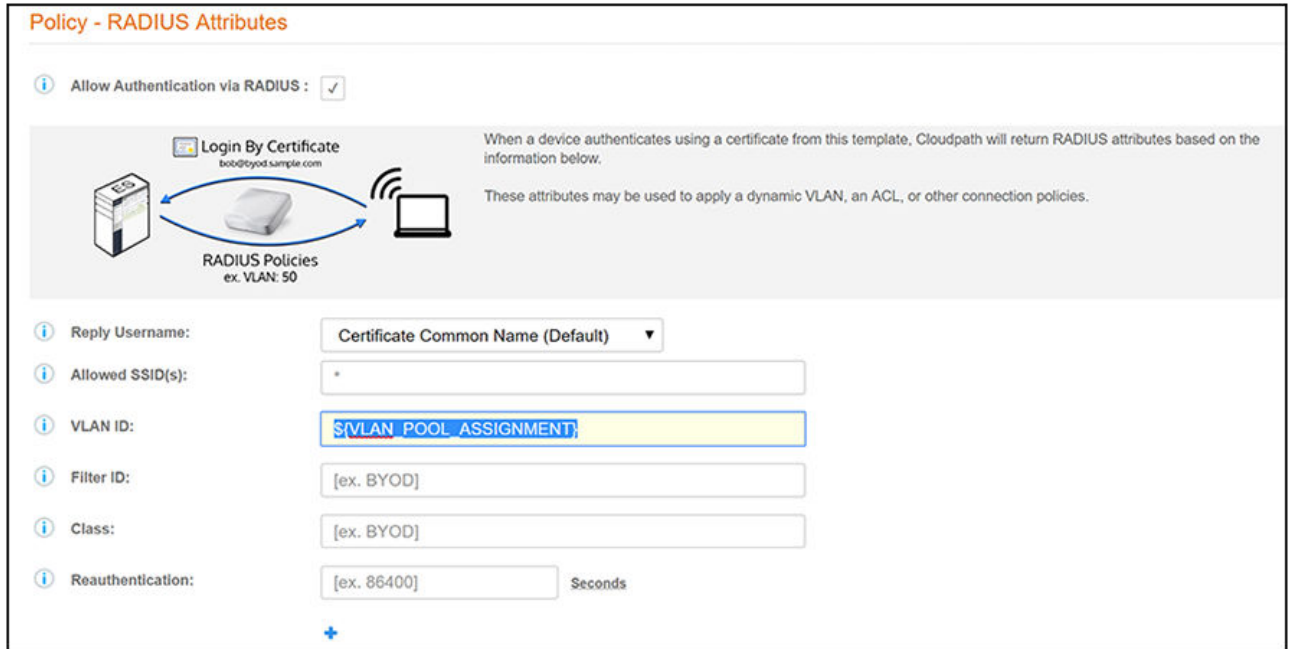
FIGURE 56 Certificate Template VLAN Variable Setting
