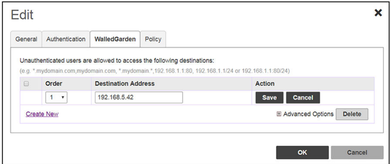
FIGURE 96 Walled Garden Configuration for Unleashed
